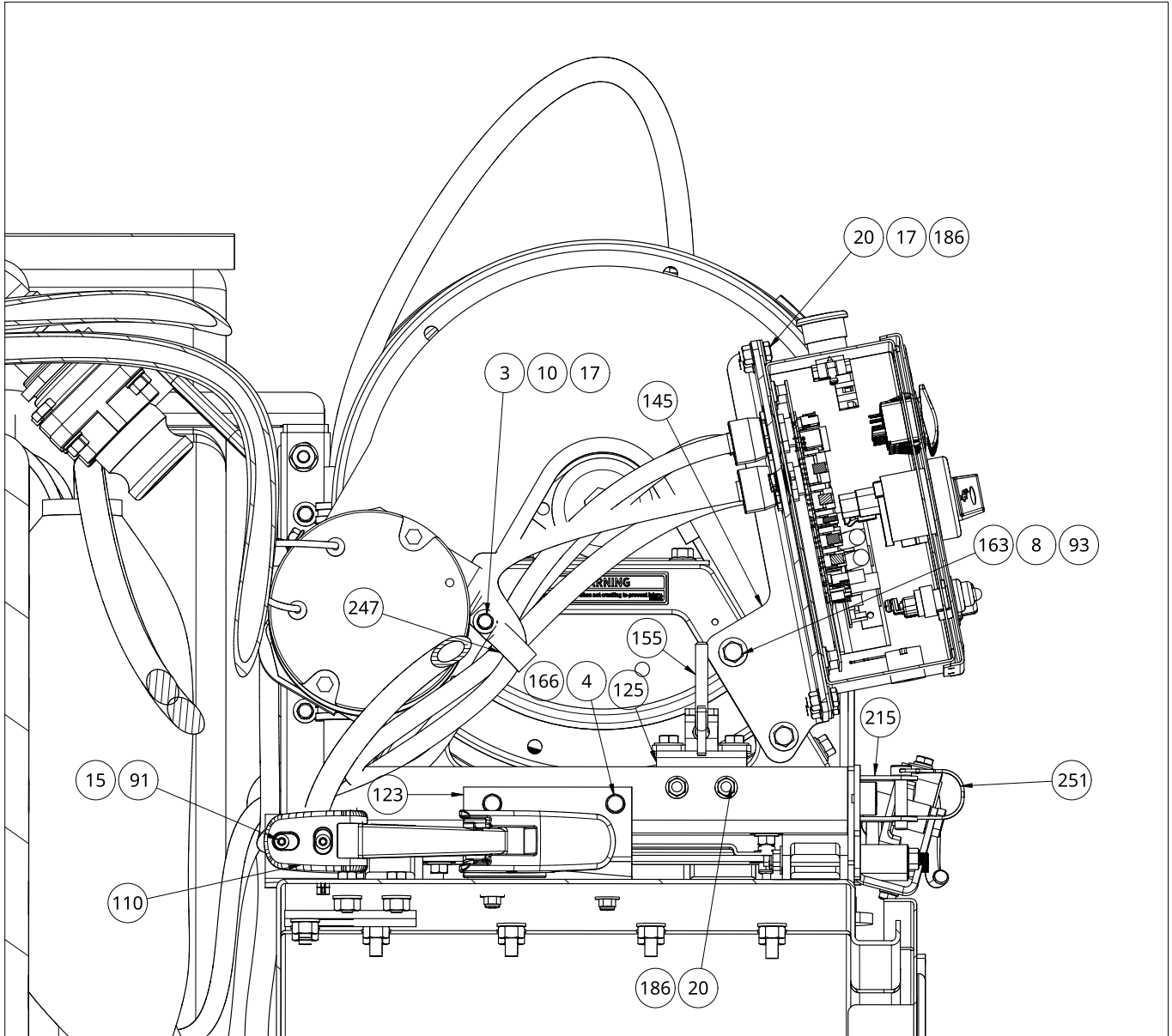
DETAIL D SCALE 1:2
