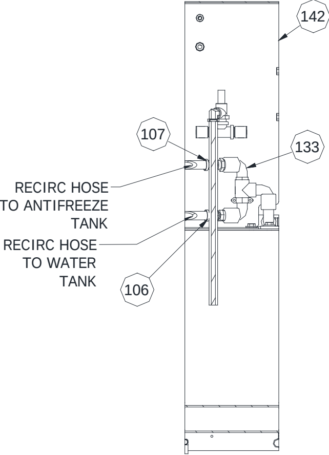
VIEW AA-AA
