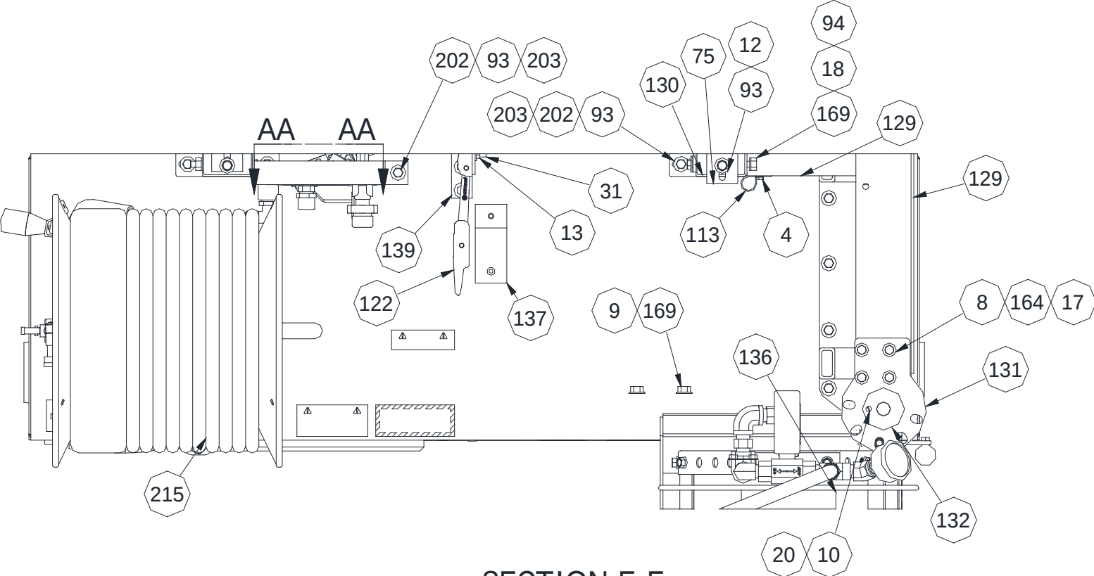
SECTION E-E
