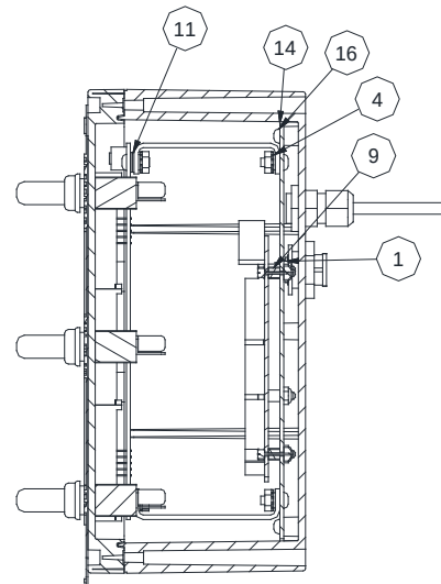
SECTION C-C
