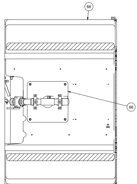
SECTION C-C
