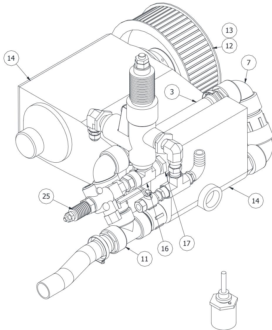
79953920 Pulsator (High Flow Version)
